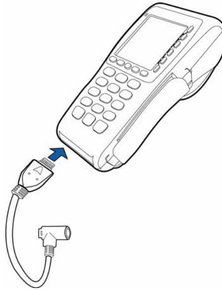
Figure 4 Power Adapter Cable Connection to a V×670 Terminal
