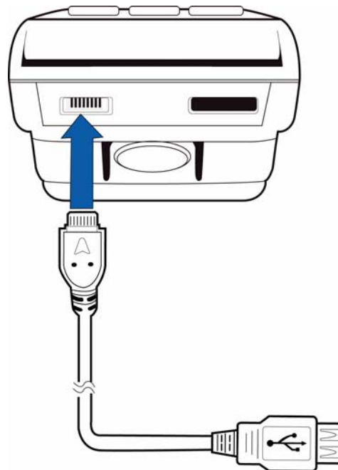
Figure 5 USB Host Cable Connection to a V×670 Terminal
