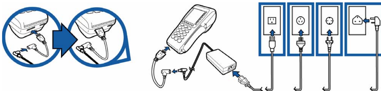
Figure 19 V x 670 Power Pack Connection
