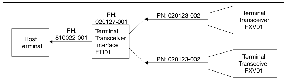
Figure 4-2. Extending basic coverage
