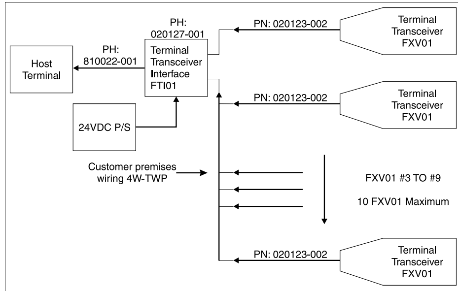
Figure 4-3. Large area coverage
