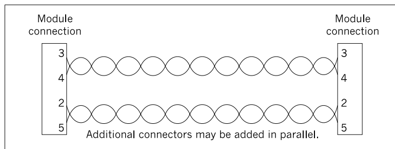
Figure 4-4. Premises wiring diagram
