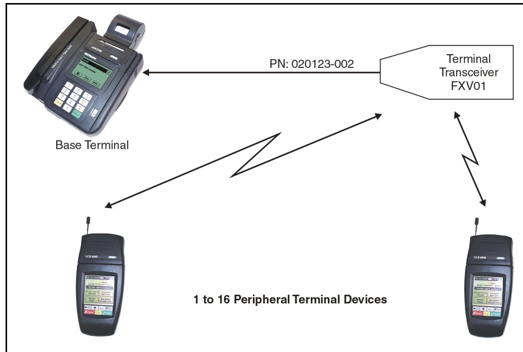
Figure 4-1. Basic configuration
