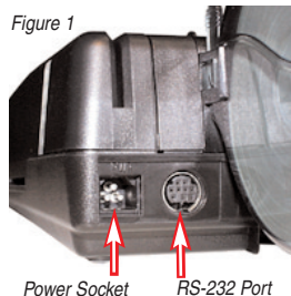
Power Socket RS-232 Port
