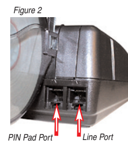
PIN Pad Port Line Port
