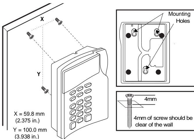
Figure 2 Wall-mounting a Terminal
