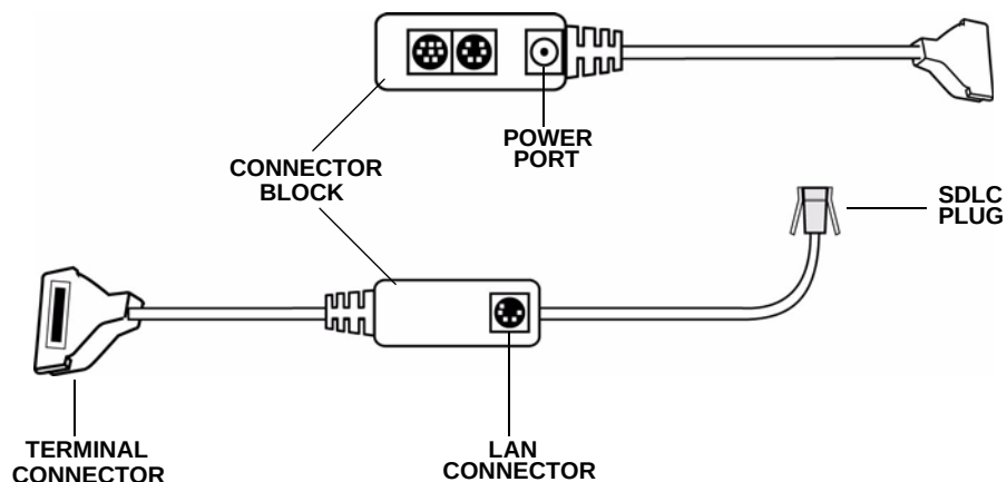
Figure 21 Multiport Cable: Front and Rear
