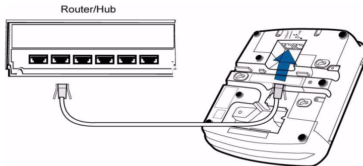
Figure 24 Ethernet Connection
