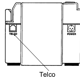
Figure 3-9. Telephone Connection
