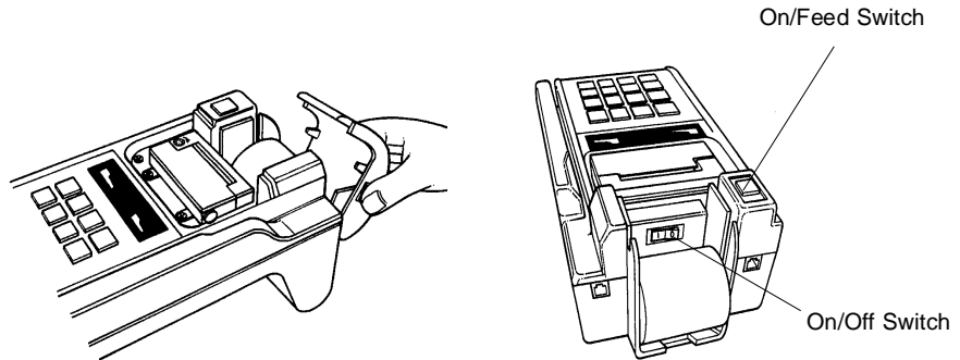
Figure 3-8. TRANZ 460 Battery Switch
